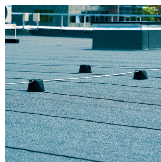
Stropodachy wentylowane
